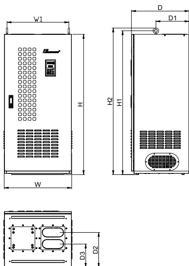
(c) 160KW~200KW 规格尺寸(柜机)
